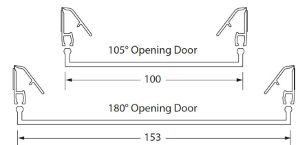
Pivot Door Installation
