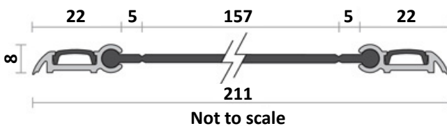
FingerKeeper Industrial - RP62 standard (measurements in mm)
