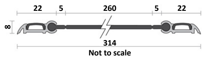
FingerKeeper Industrial - RP62 wide (measurements in mm)
