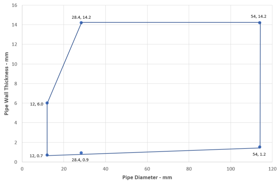
Steel Pipes with Elastomeric Insulation - C/C
